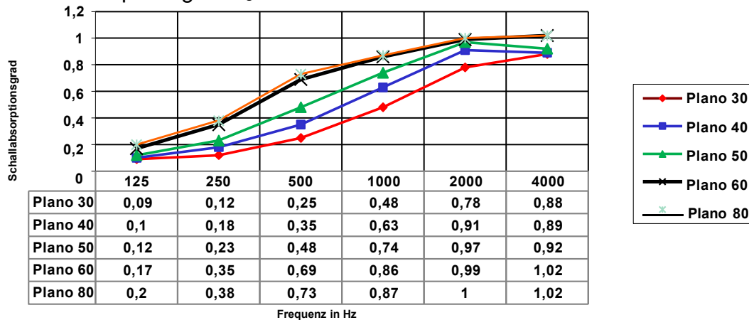
Schallabsorptionsgrad \alpha_s
