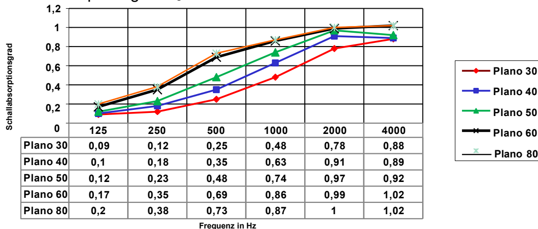
Schallabsorptionsgrad \alpha_s
